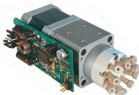
10 PORT INTEGRATED MOTOR/VALVE 1/16" PEEK ZDV fittings
